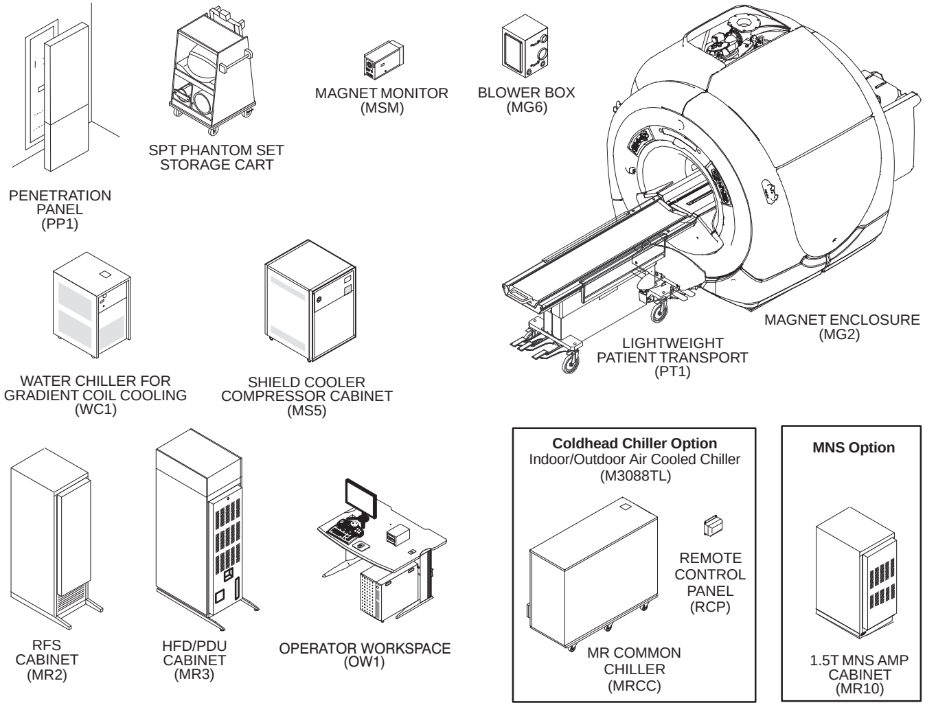
ILLUSTRATION 10-1 SIGNAL EXCITE HDx & HDi 1.5T SYSTEM
